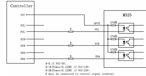
Figure 4: Connections to difference control signal
